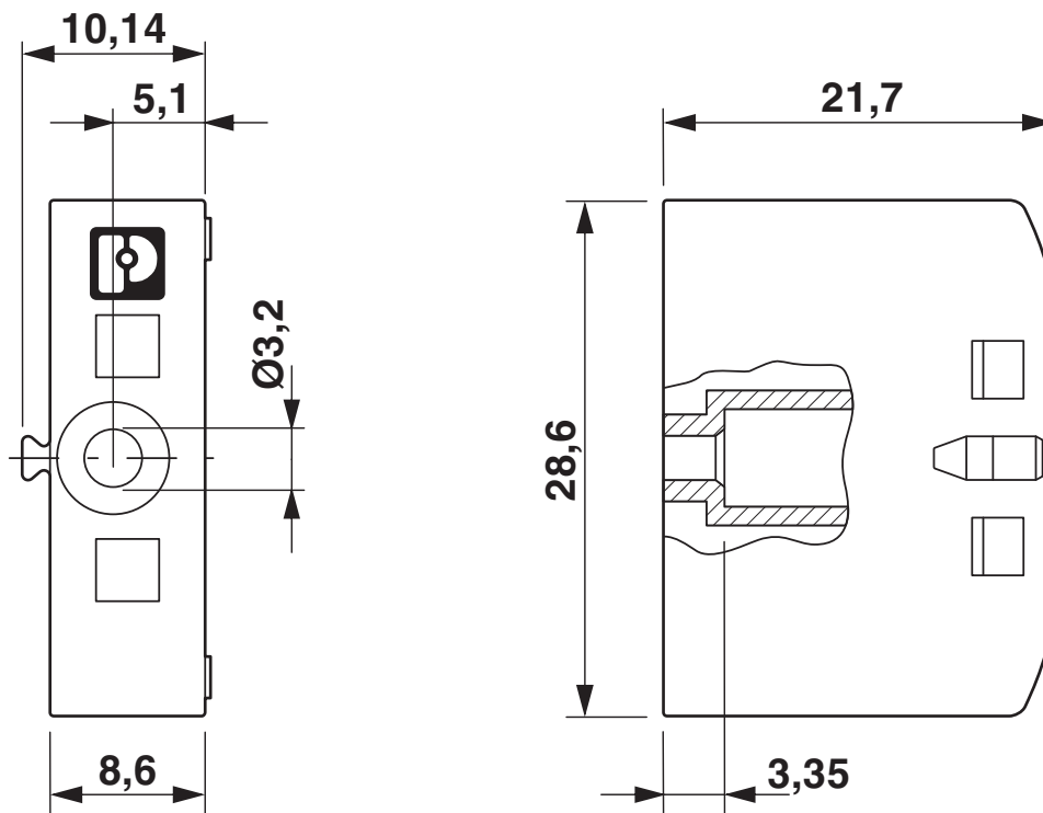
Dimensional drawing
