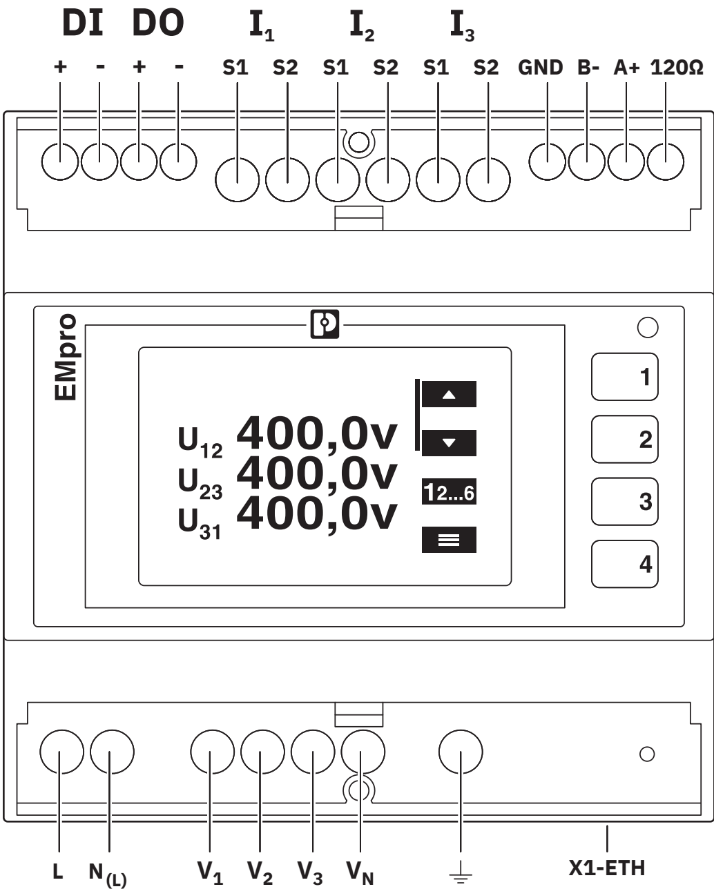
Connection diagram
