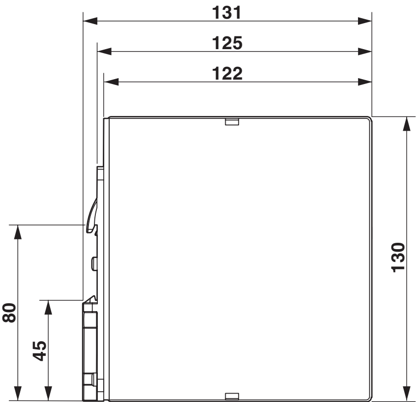
Dimensional drawing
