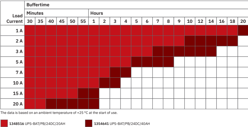
TRIO-UPS-2G buffer times for lead battery modules
