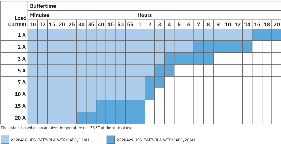
TRIO-UPS-2G buffer times for VRLA-WTR battery modules
