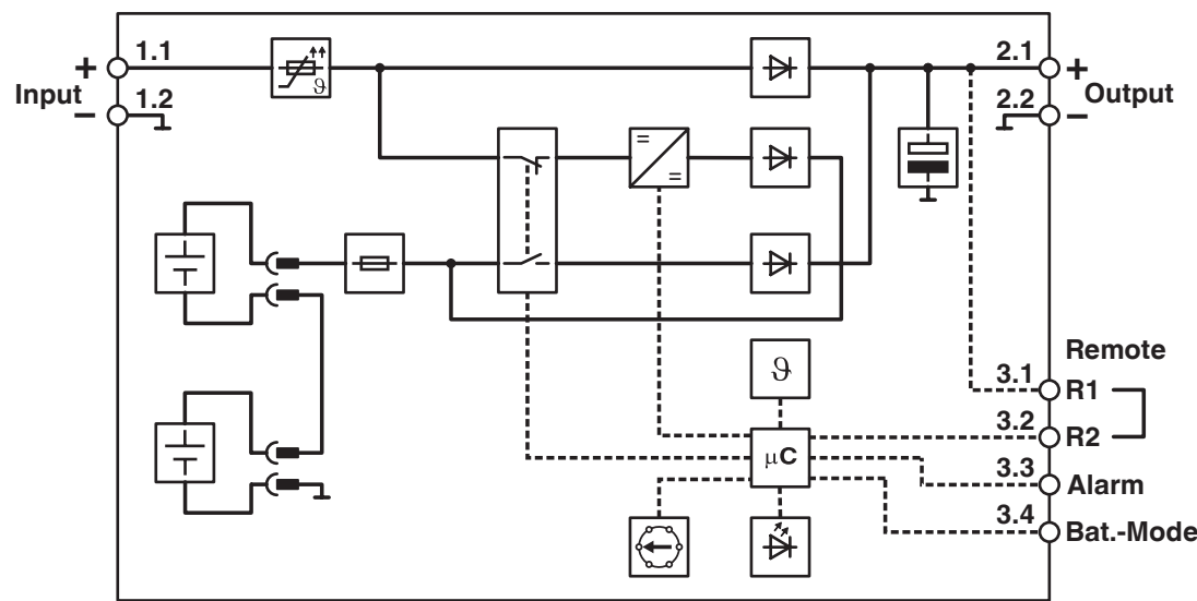
Block diagram
