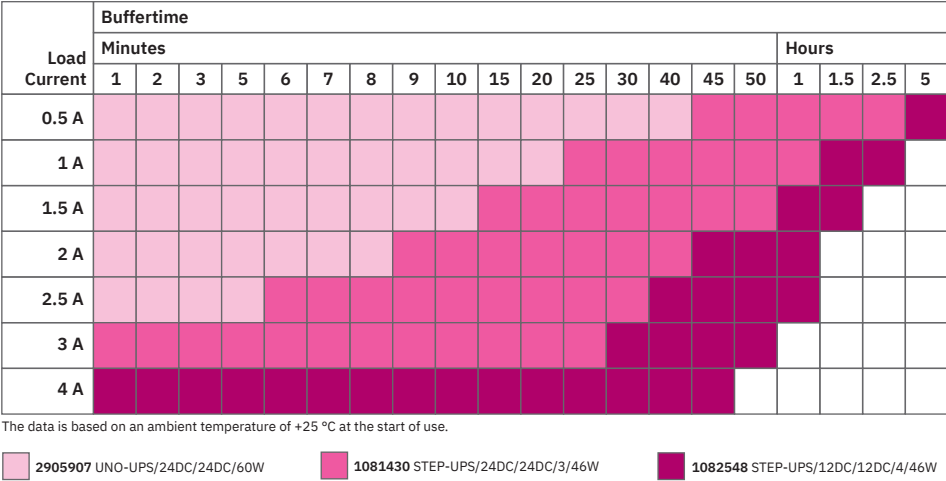
Buffer times for UNO DC UPS with integrated battery
