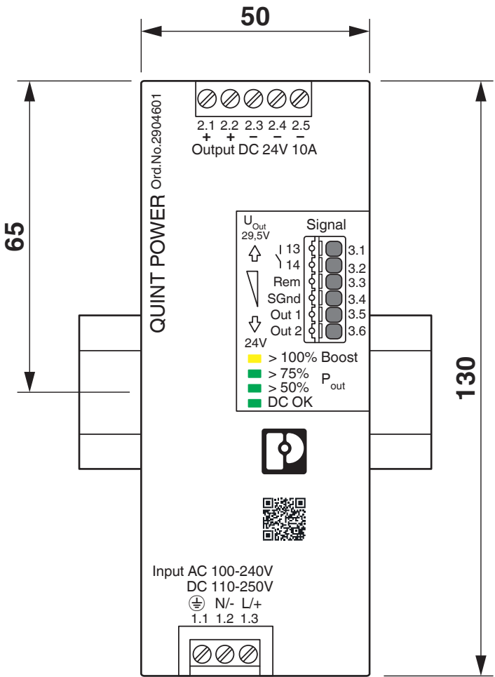
Dimensional drawing
