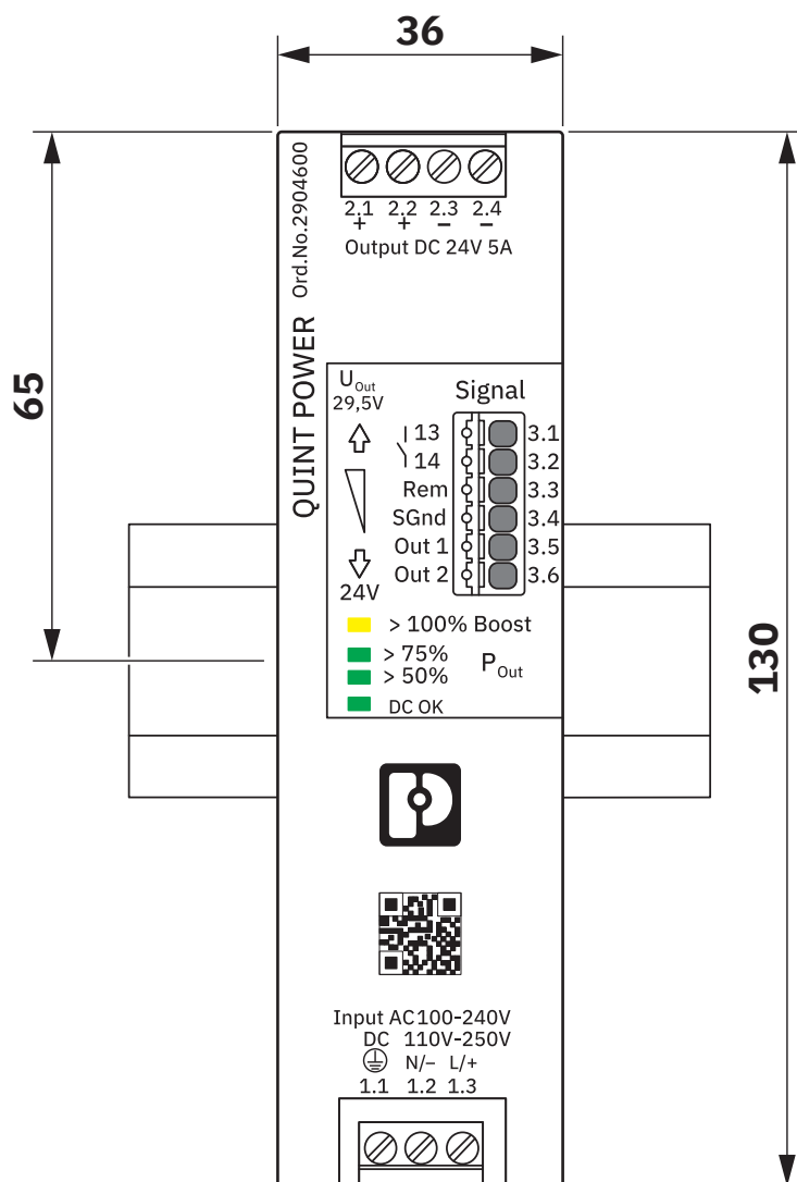
Dimensional drawing
