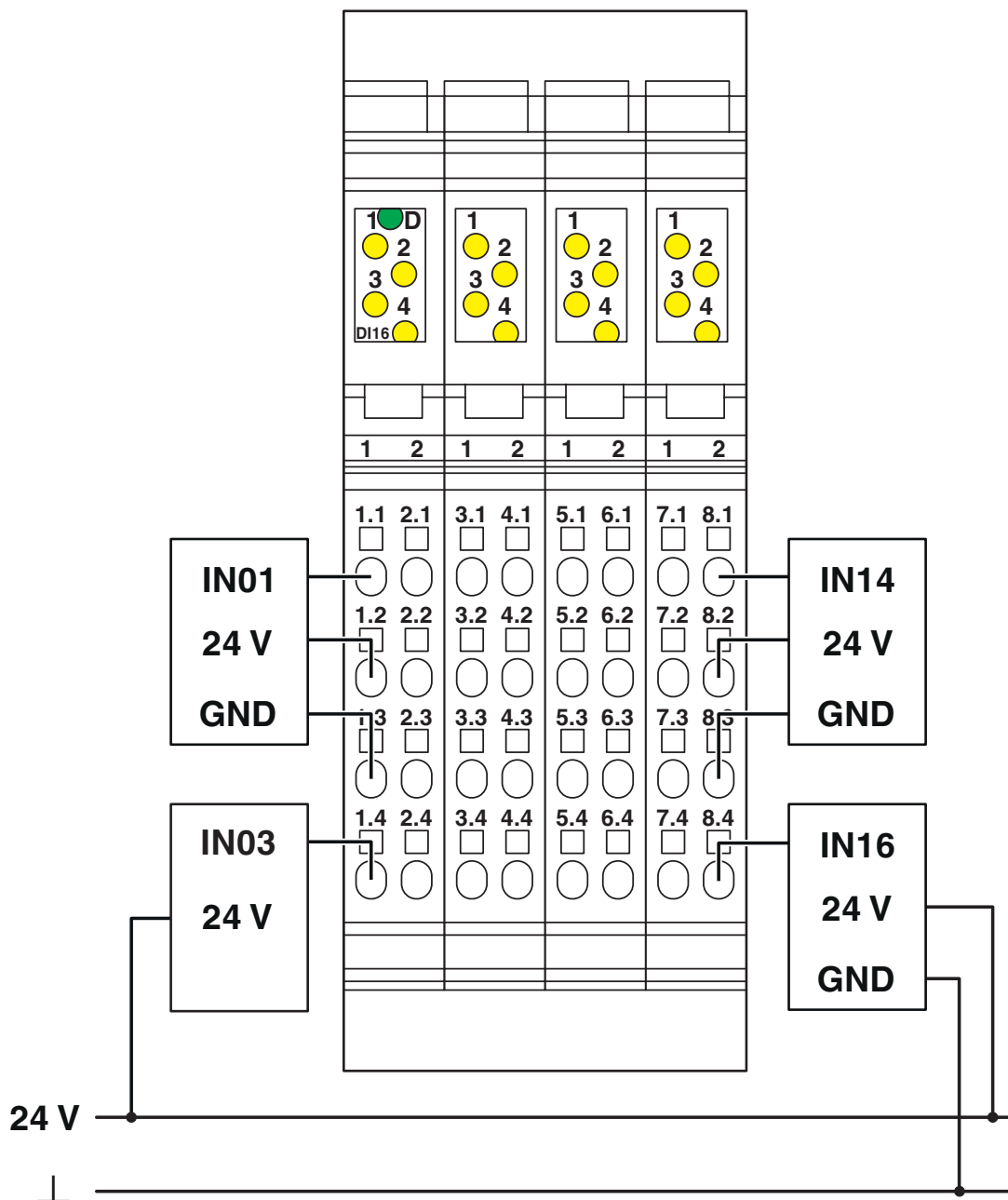
Connection diagram
