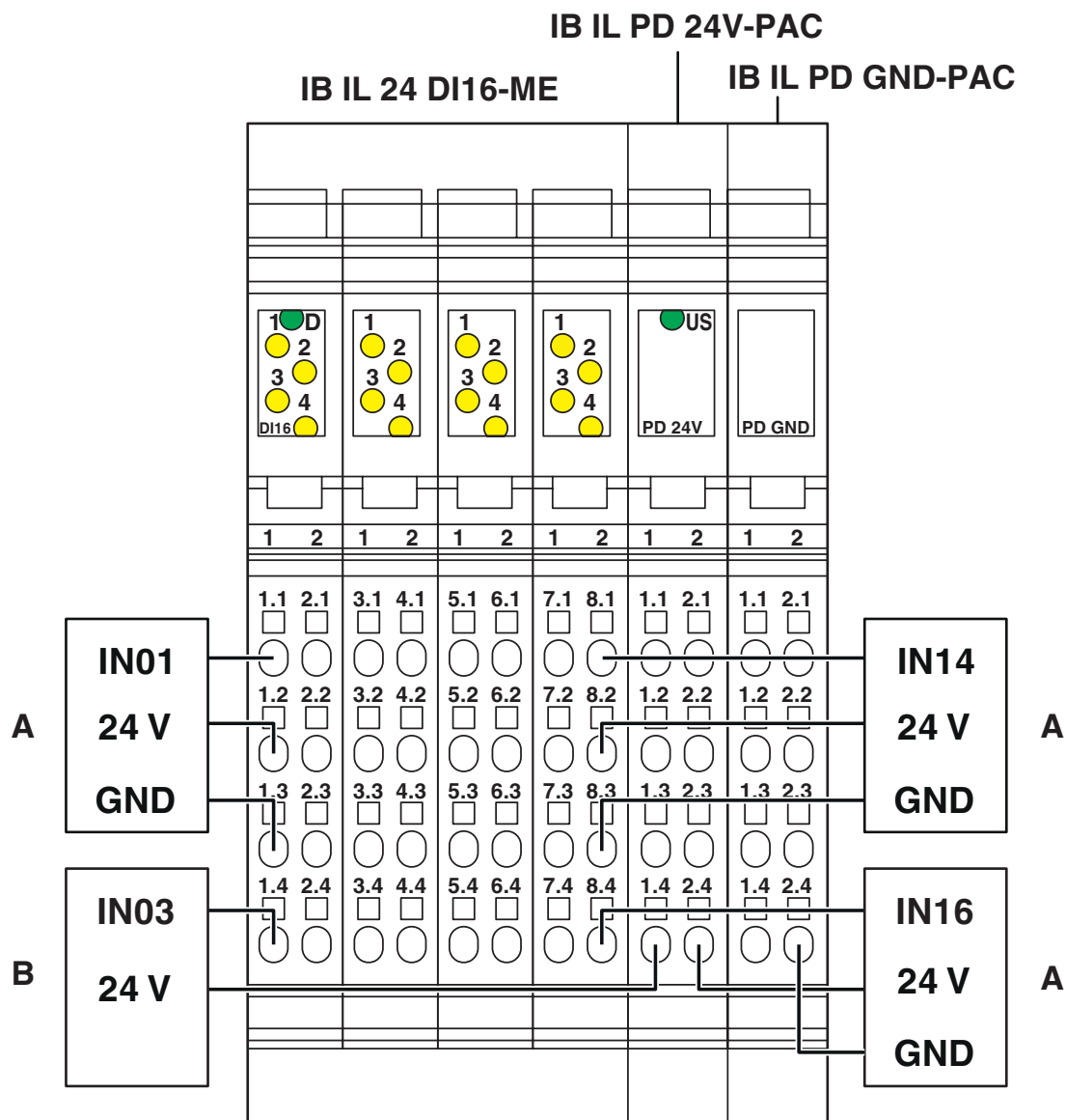
Connection diagram
