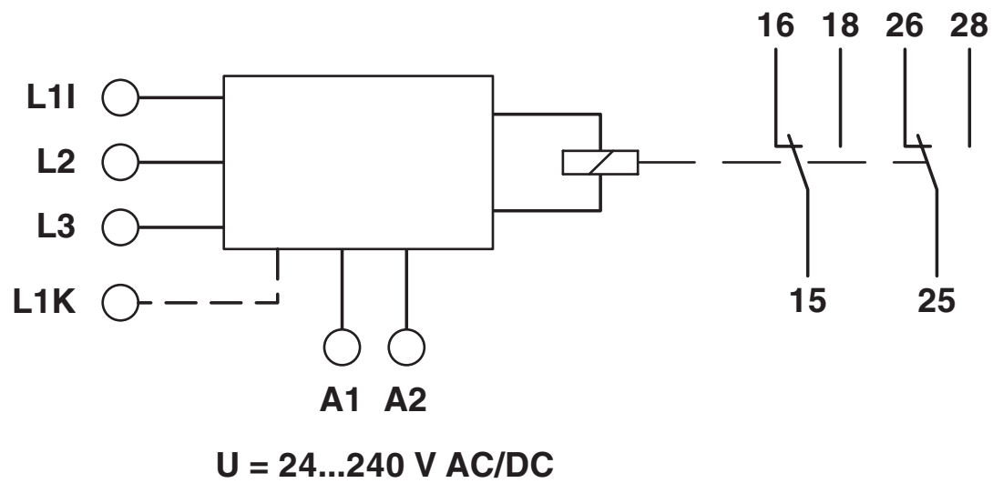
Block diagram
