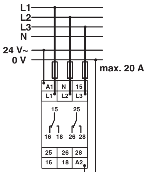
Connection diagram
