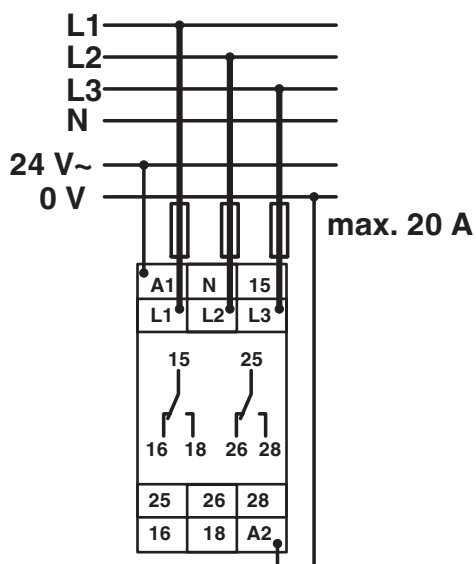
Application drawing
