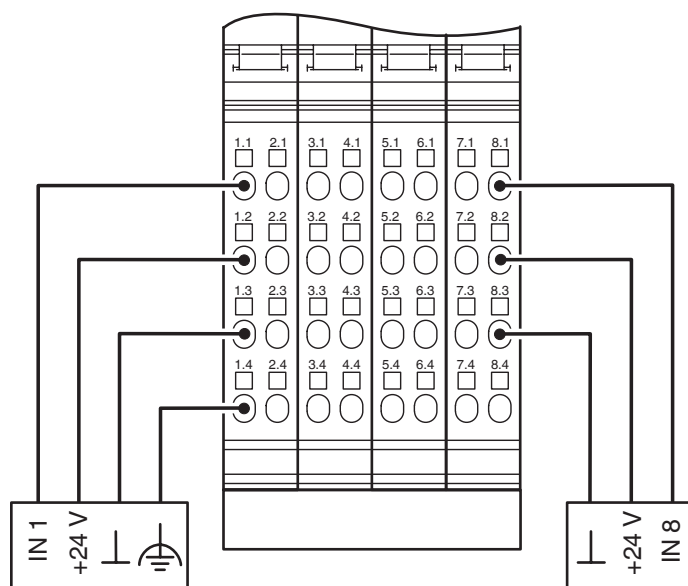
Connection diagram
