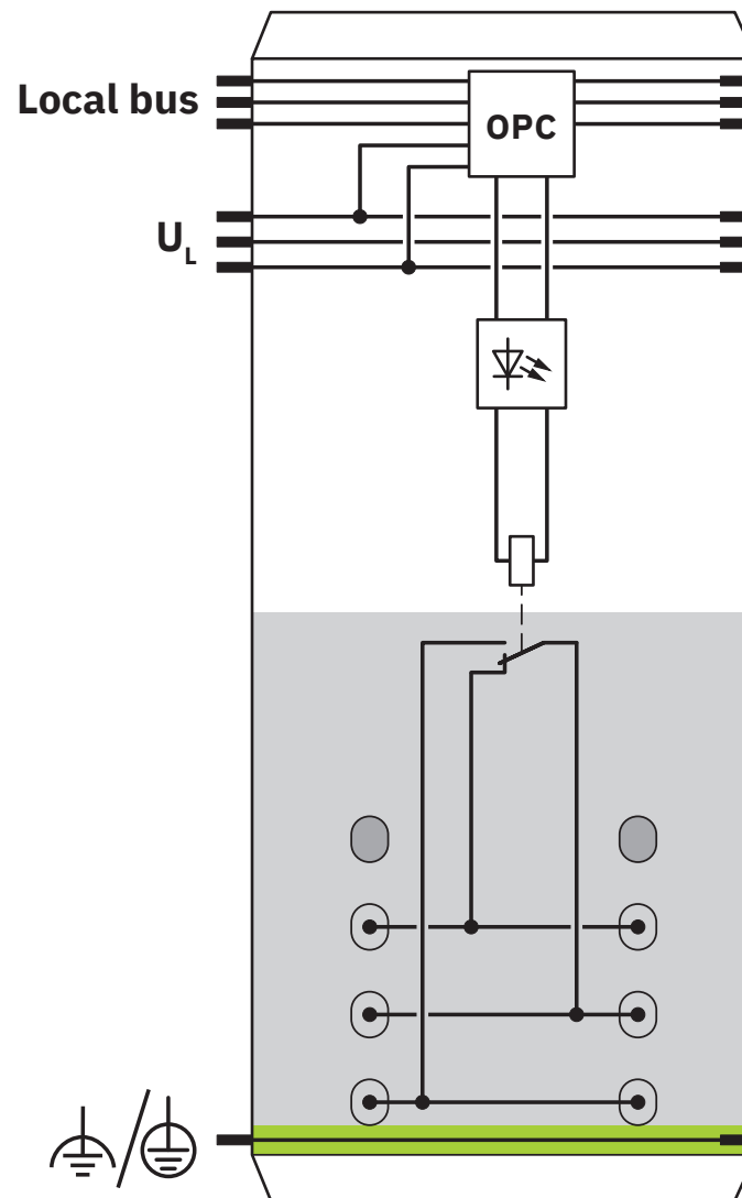
Block diagram
