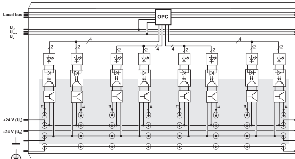
Block diagram
