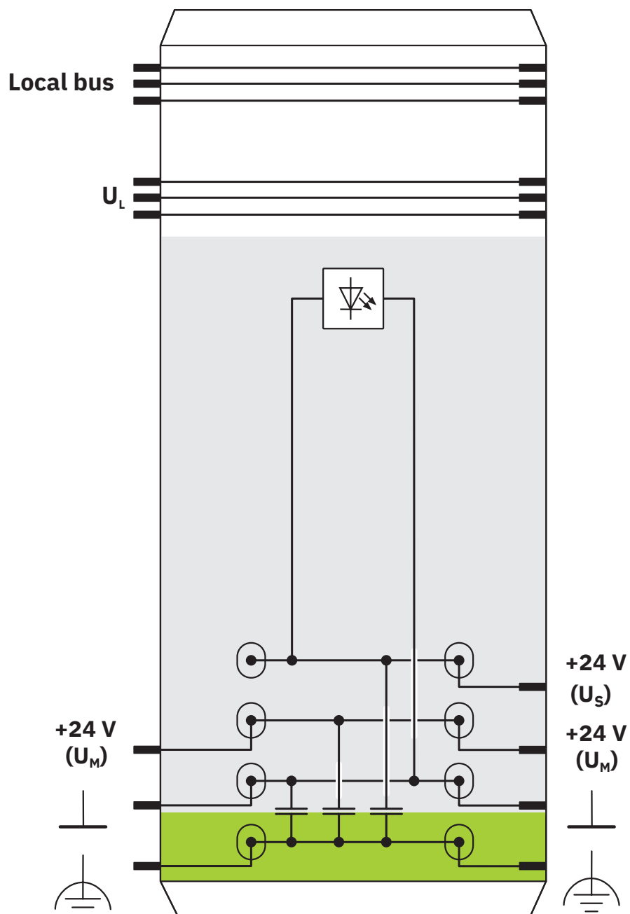
Internal wiring of the terminal points
