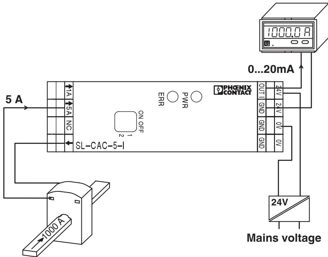
Application drawing
