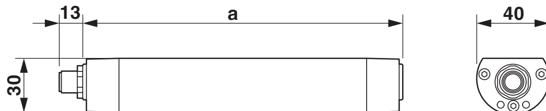
Dimensional drawing
