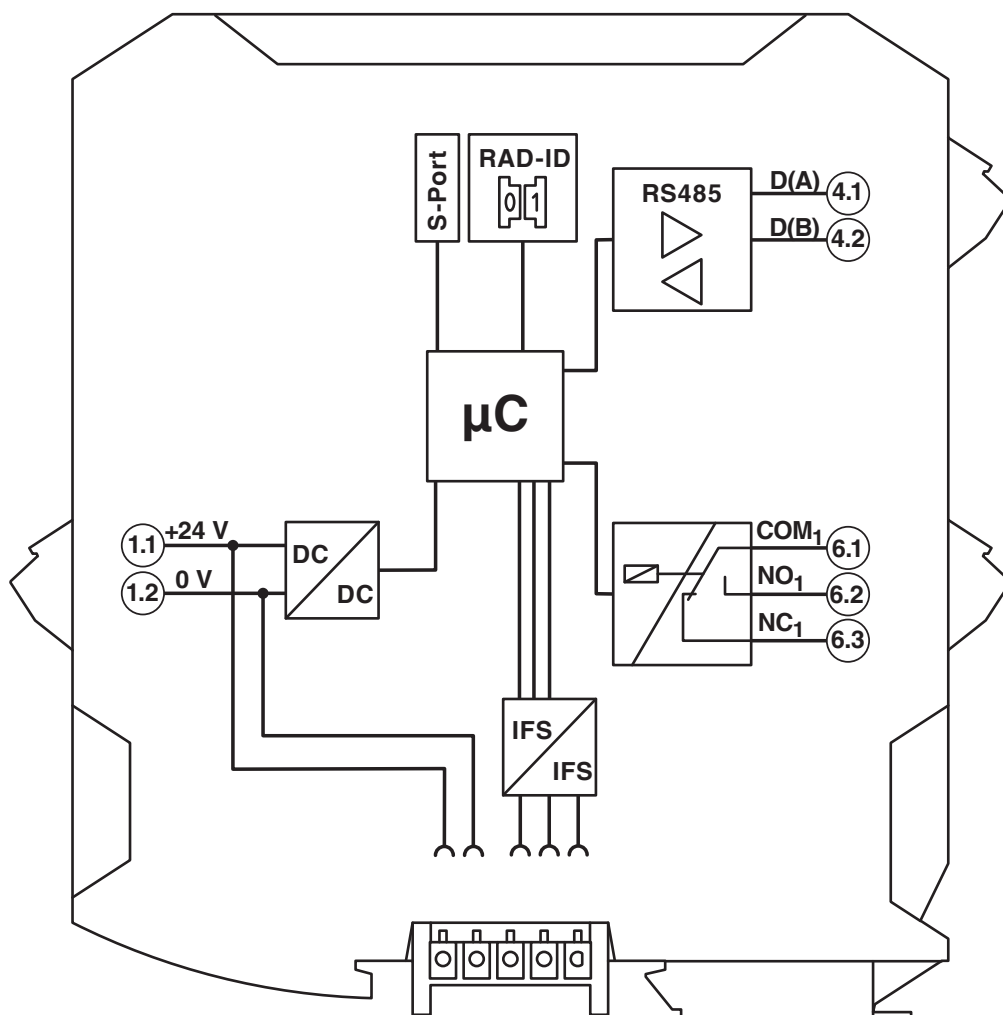
Circuit diagram
