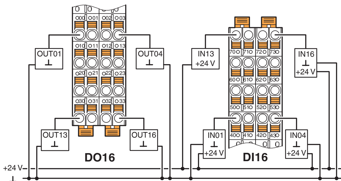
Connection diagram
