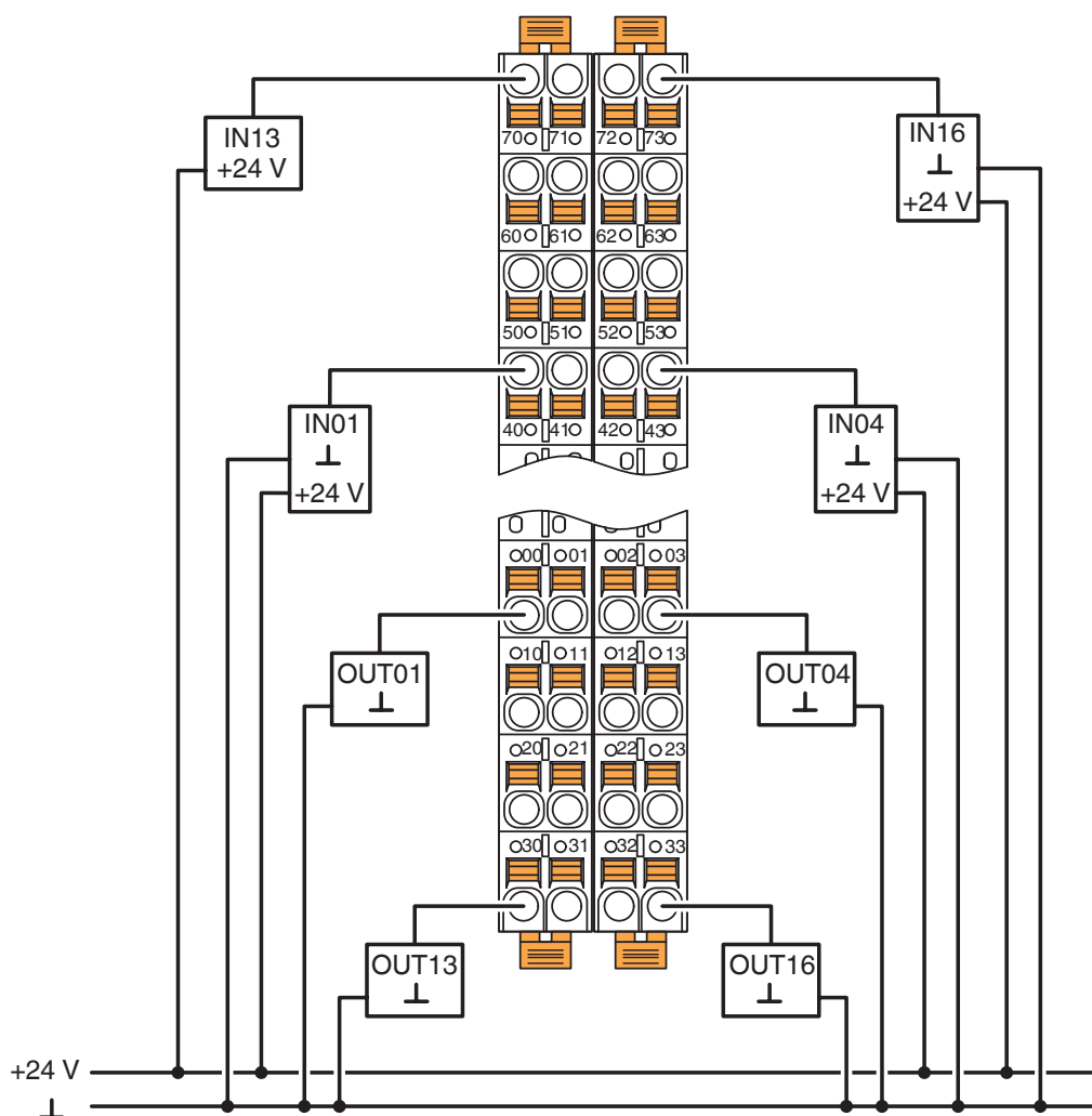
Connection diagram
