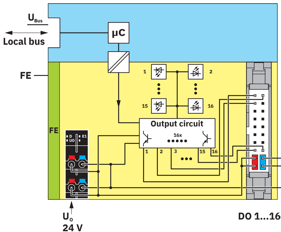
Block diagram
