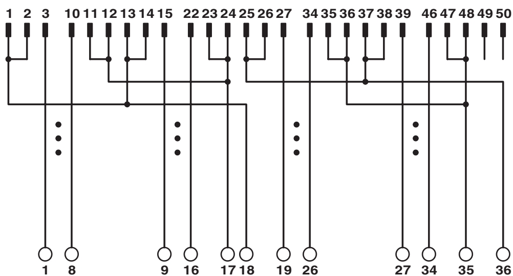
Connection scheme VIP-2/.../FLK50/AB-1756
