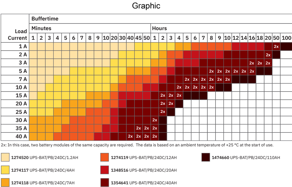
QUINT DC UPS buffer times for PB battery module
