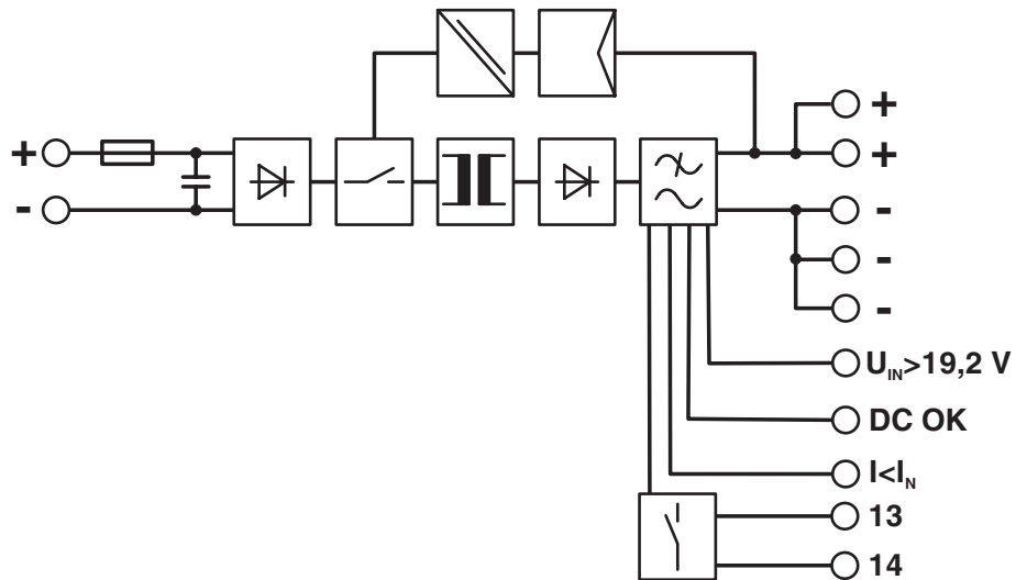
Block diagram
