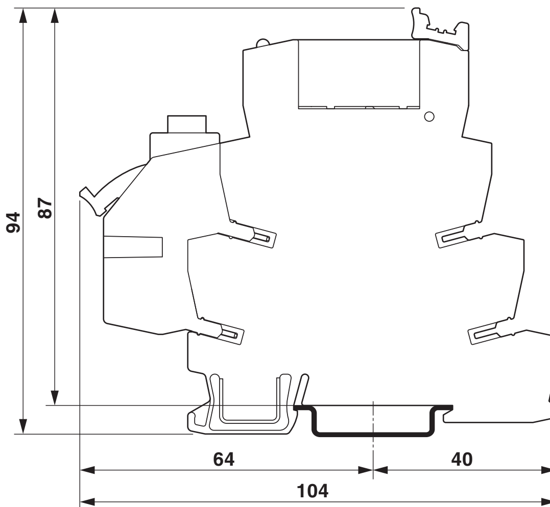
Dimensional drawing
