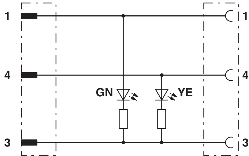
Circuit diagram
