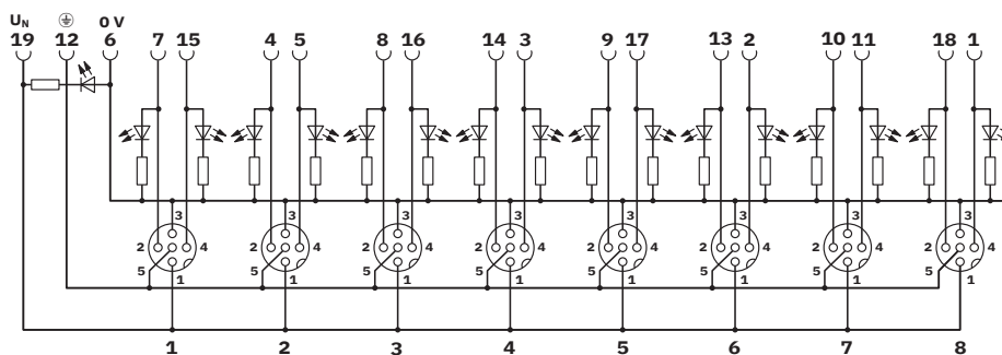
Circuit diagram
