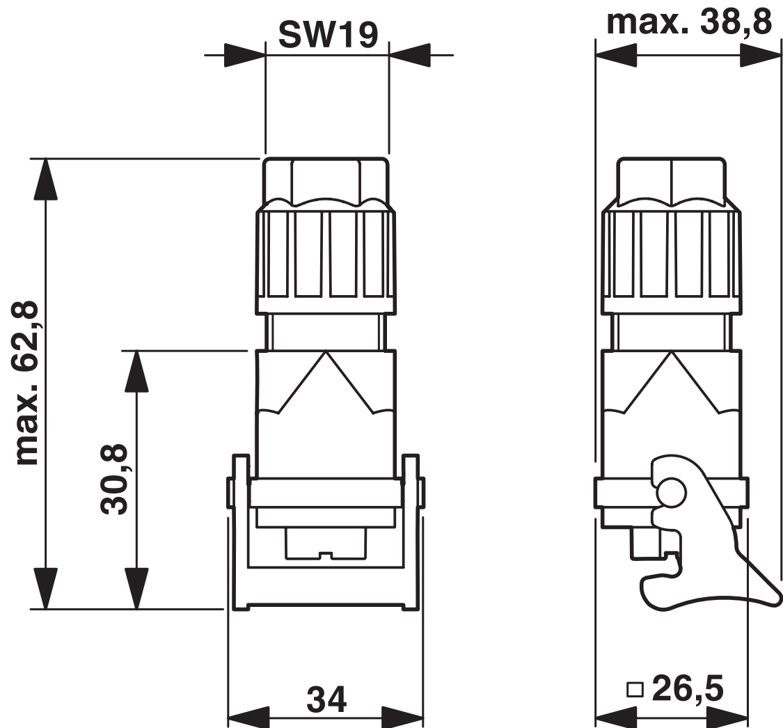
Dimensional drawing
