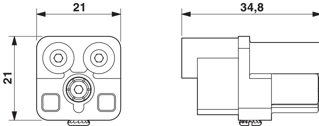
Dimensional drawing
