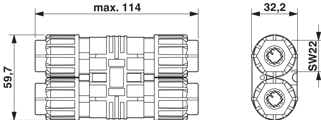
Dimensional drawing
