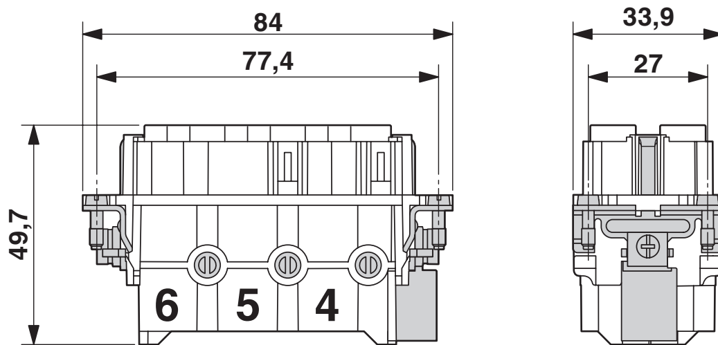
Dimensional drawing
