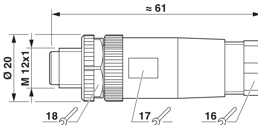
Dimensional drawing
