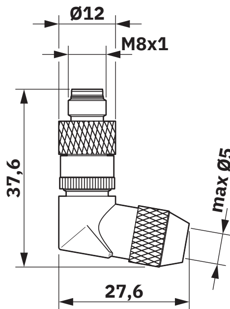
Dimensional drawing
