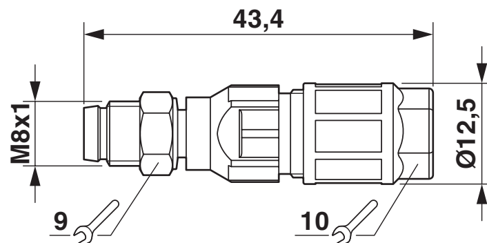
Dimensional drawing
