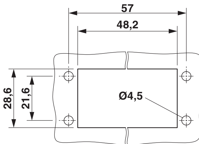
Dimensional drawing
