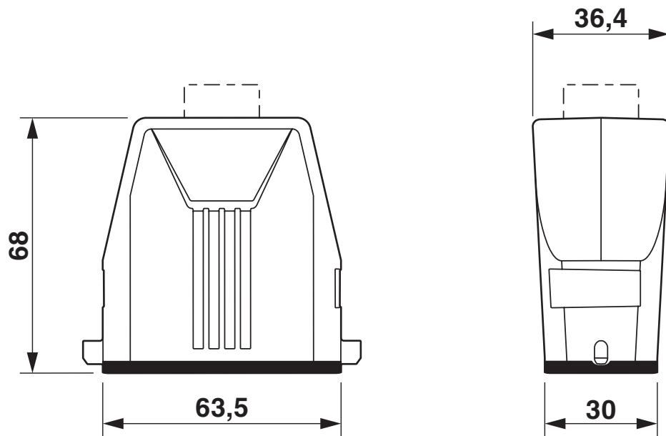
Dimensional drawing
