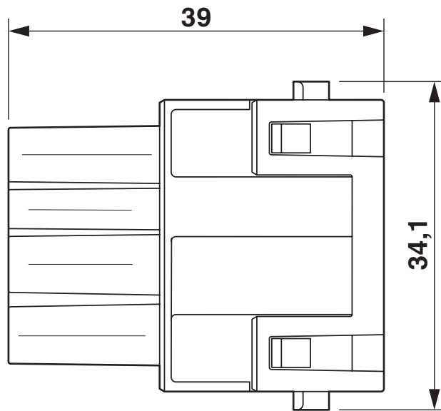
Dimensional drawing
