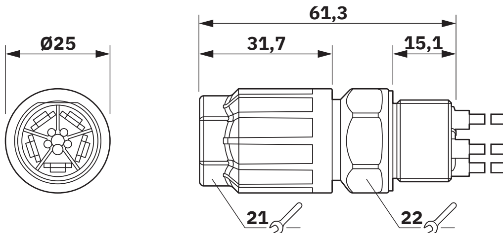
Dimensional drawing
