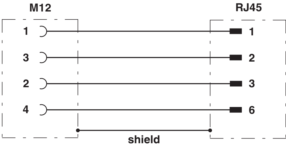
Circuit diagram
