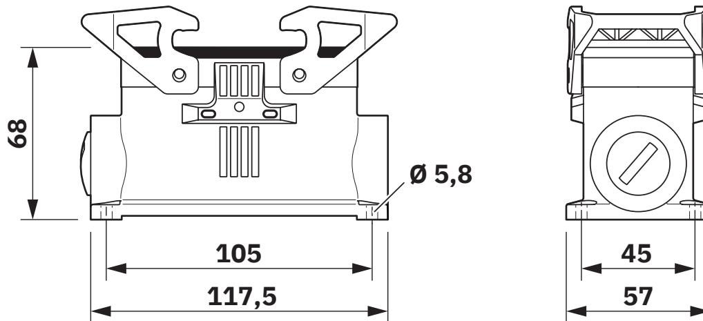
Dimensional drawing
