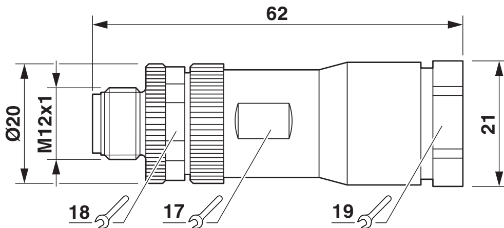
Dimensional drawing
