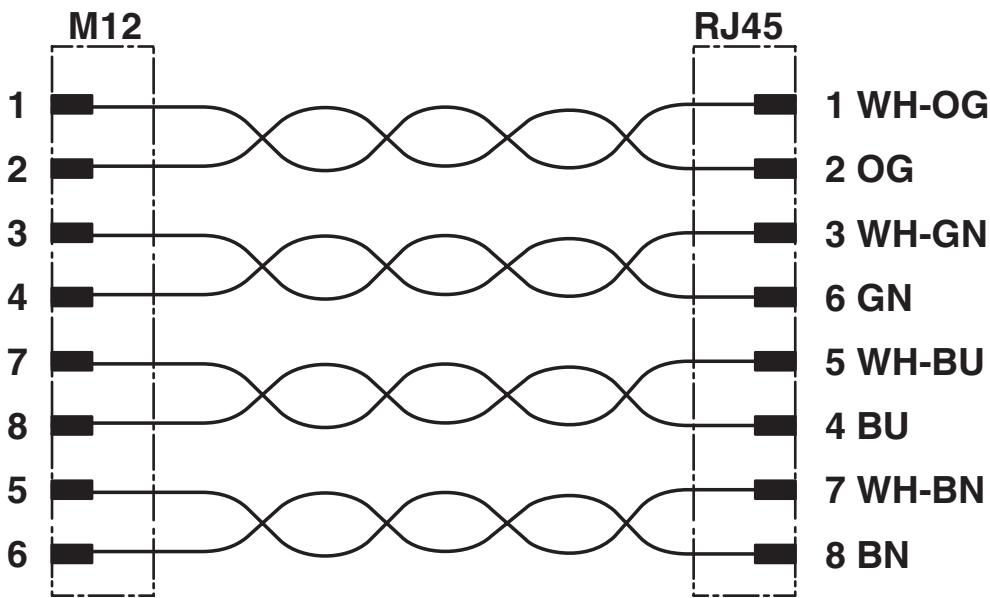
Circuit diagram
