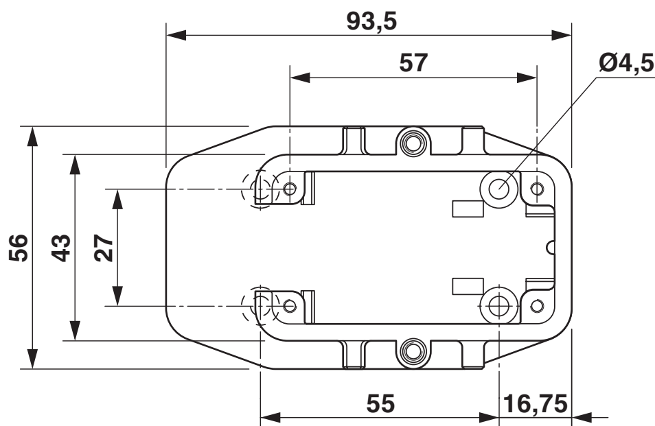
Dimensional drawing
