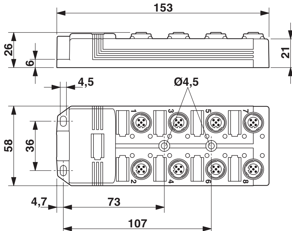
Dimensional drawing
