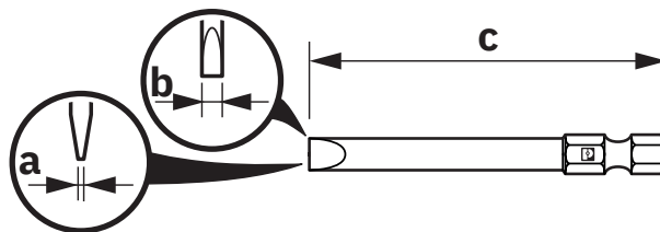
Dimensional drawing
