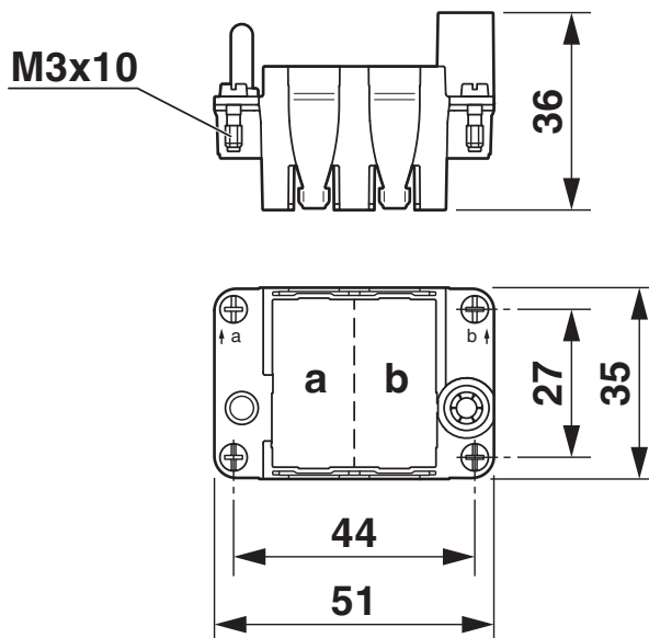
Dimensional drawing
