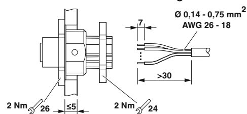
Functional drawing
