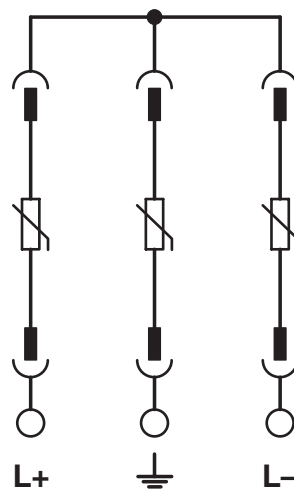
Circuit diagram
