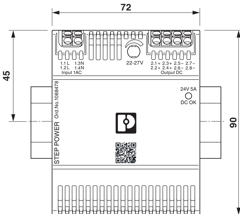
Dimensional drawing
