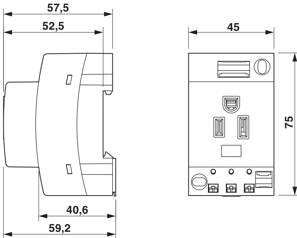
Dimensional drawing
