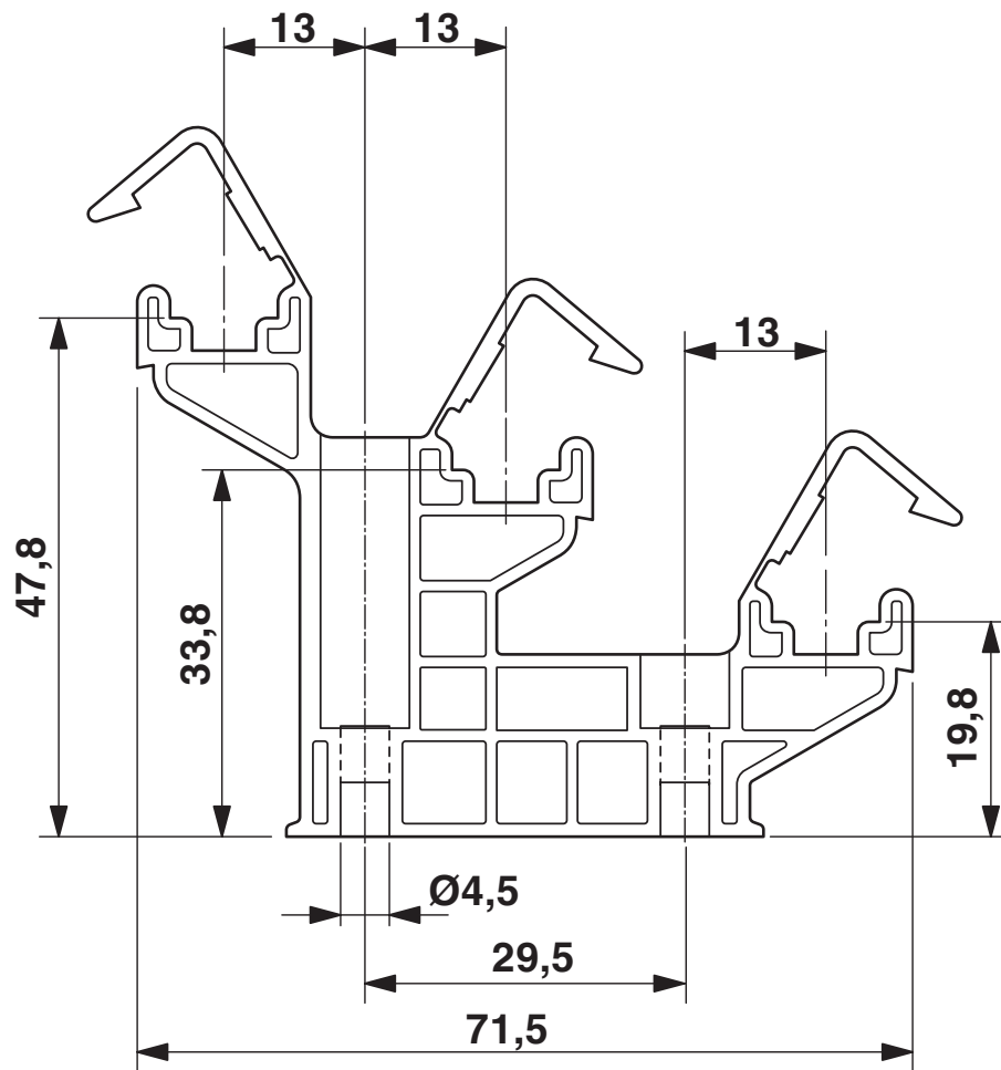
Dimensional drawing
